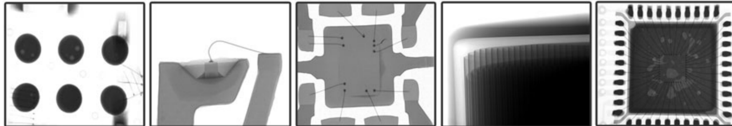
BGA
